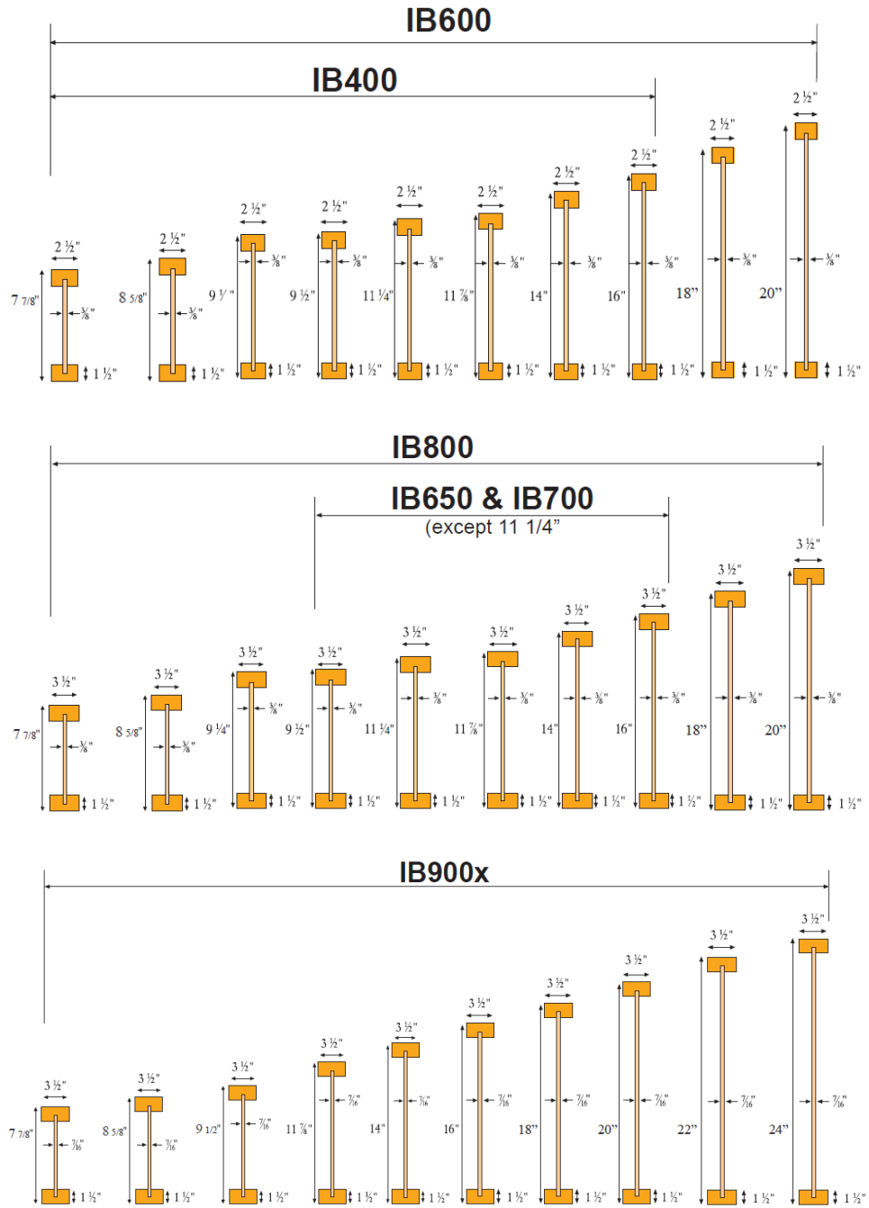
FIGURE 1 – I-JOIST ILLUSTRATIONS
