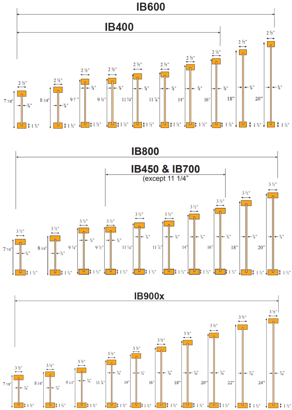
FIGURE 1 – I-JOIST ILLUSTRATIONS
