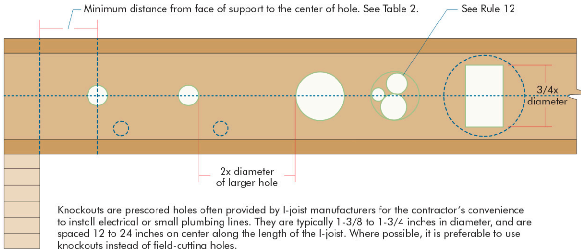
FIGURE 1—TYPICAL HOLES
